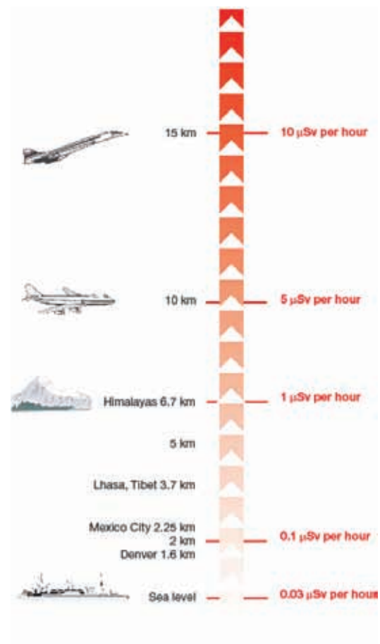
FIG.5. CoFsmic radiation and dose rates of exposure.
